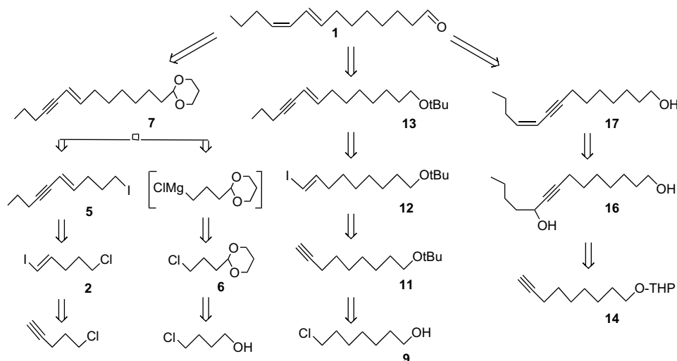
Scheme 1. Retrosynthetic analysis of aldehyde 1 of the female-produced contact sex pheromone of the horse-chestnut leafminer, C. ohridella .
