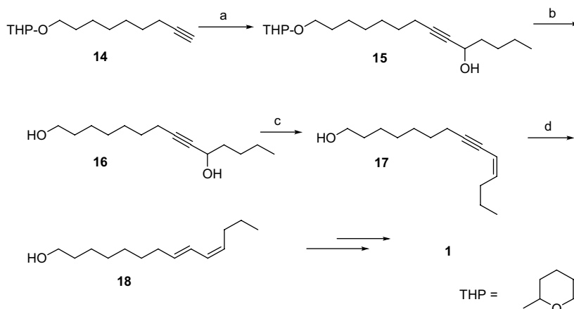
Scheme 4. Synthesis of precursor 18 ; (a) 1. n -BuLi, THF, -30\text{ }^{\circ}\text{C} \rightarrow 0\text{ }^{\circ}\text{C} , 2. pentanal, THF, -25\text{ }^{\circ}\text{C} (84%, two steps); (b) TsOH, MeOH (85%); (c) \text{KHSO}_4 , Büchi B-580 vacuum oven 155\text{--}165\text{ }^{\circ}\text{C}/0.2\text{ mmHg} (40%); (d) LAH, diglyme-THF, 117\text{--}121\text{ }^{\circ}\text{C} for 29 h (71%).
