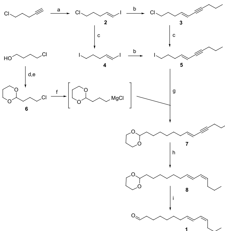
Scheme 2. Synthesis of 1 employing the C5+C5+C4 strategy; (a) 1. DIBAH, hexane, 50 °C; 2. I 2 , THF, −40 °C (63%, two steps); (b) n -PrC≡CMgBr, 3 mol % Pd(PPh 3 ) 4 , THF (89% for 3 ; 99% for 5 ); (c) NaI, CH 3 COC 2 H 5 (90% for 4 ; 95% for 5 ); (d) PCC, CH 2 Cl 2 ; (e) HOCH 2 CH 2 CH 2 OH, TsOH, toluene (47%, two steps); (f) Mg, C 2 H 5 I, THF; (g) CuBr, THF, −20 °C → 10 °C (80%); (h) 1. dicyclohexylborane, THF, 2. glacial AcOH, 3. 6 N NaOH, 4. 30% H 2 O 2 (83%); (i) HCO 2 H–CCl 3 CH 3 (72%).
