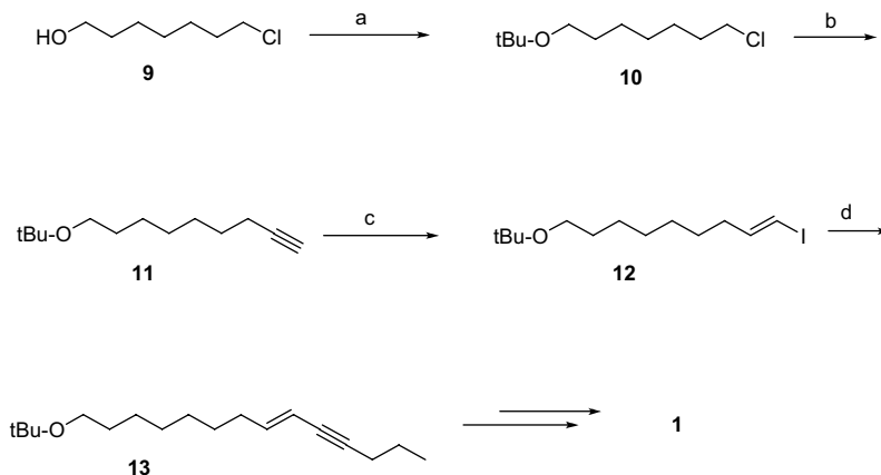
Scheme 3. Synthesis of the key intermediate 13 according to C7+C2+C5 strategy; (a) isobutylene, Amberlyst H-15, hexane (84%); (b) LiC≡CH·EDA, DMA, –5 °C → rt, (82%); (c) 1. DIBALH, hexane, 53 °C, 2. I 2 , THF, –47 °C (61%, two steps); (d) n -PrC≡CMgBr, 3 mol % Pd(PPh 3 ) 4 , THF (94%).
